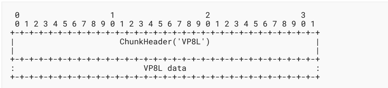
Figure 6: 'VP8L' Chunk
