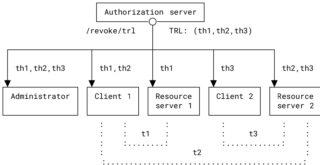
Figure 1: Protocol Overview
